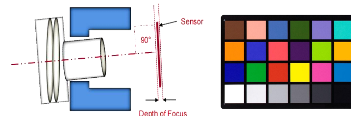
Ideal Alignment and Centering Clear Image
