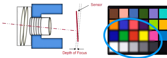
Poor Tilt Control Blurred Image
